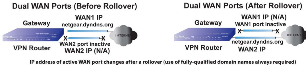
Figure B-7 Rollover with Dual WAN Ports
