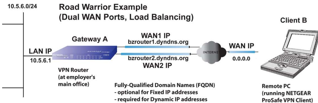
Figure B-12 Road Warrior, Dual WAN Ports, Load Balancing
