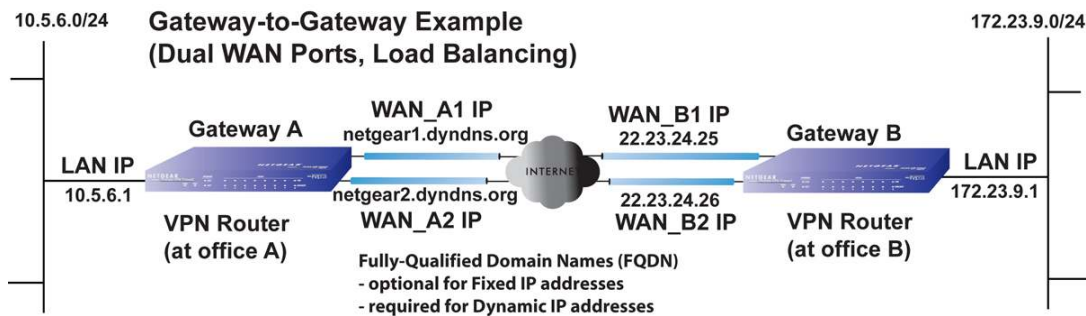
Figure B-16 Gateway-to-Gateway, Dual WAN Ports, Load Balancing
