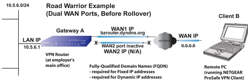
Figure B-10 Road Warrior, Dual Gateway WAN Ports
