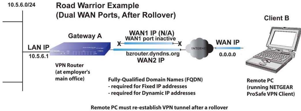
Figure B-11 Road Warrior, Dual WAN Ports, Rollover
