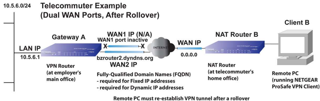
Figure B-19 Telecommuter Example
