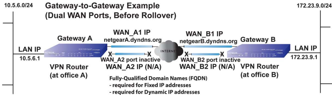
Figure B-14 Gateway-to-Gateway, Dual WAN Ports
