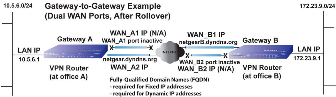
Figure B-15 Gateway to Gateway, Dual WAN Ports after Rollover
