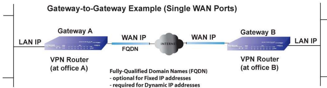
Figure 5-5 Gateway-to-Gateway Example
