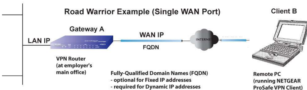
Figure 5-6 Client to Gateway VPN Tunnel
