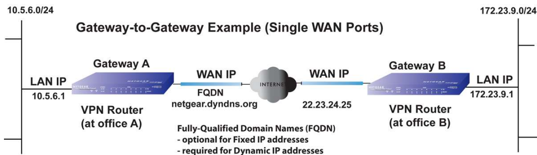
Figure B-13 Gateway-to-Gateway with Single WAN Ports
