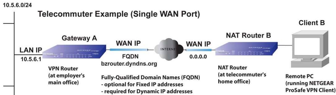
Figure B-17 Telecommuter, Single Gateway WAN Port
