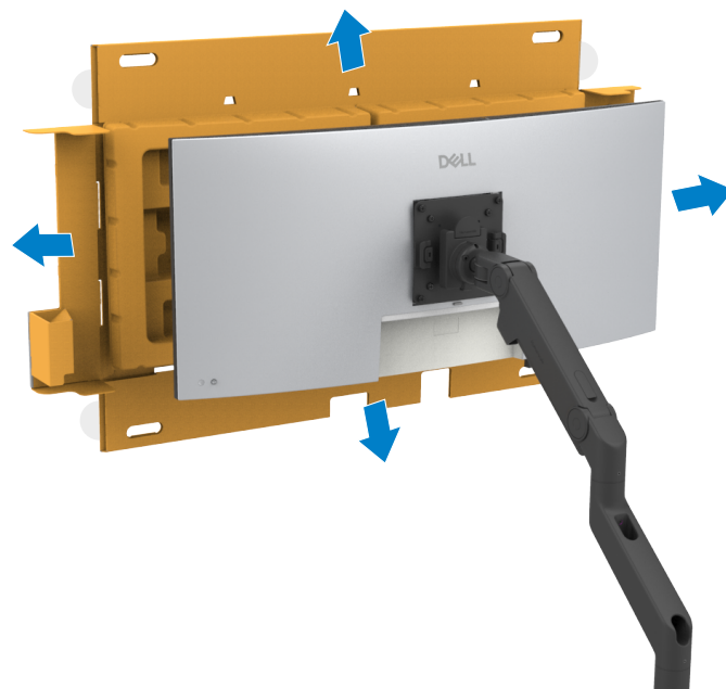
Figure 26. Remove the inner corrugated tray from the monitor
