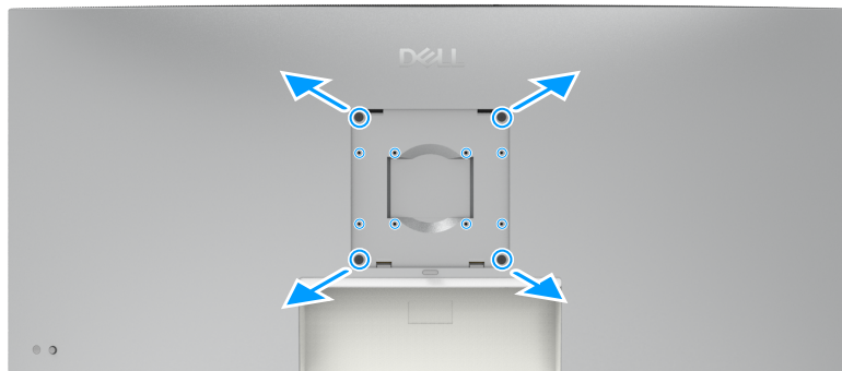
Figure 53. VESA wall mounting (optional)
