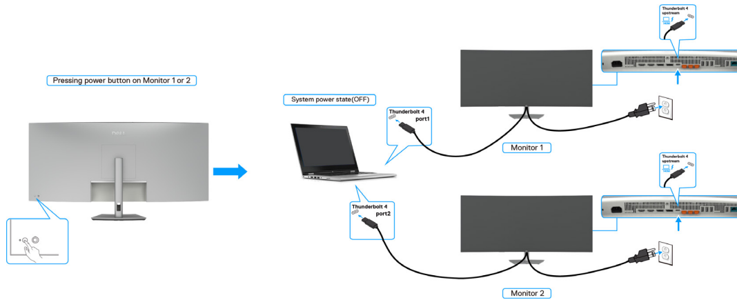
Figure 48. Pressing the power button on either monitor will turn off both monitors and the computer
