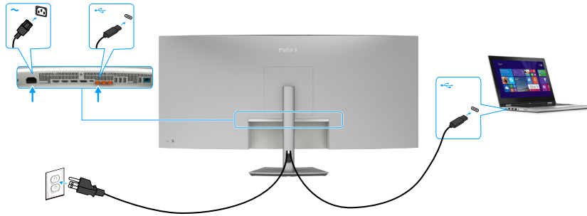
Figure 32. Connecting the USB-C cable (C to C) (Optional)
