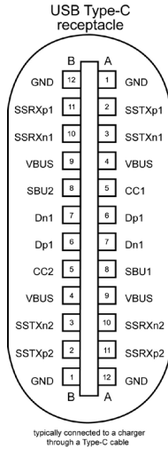
Figure 7. Thunderbolt 4/USB-C port
