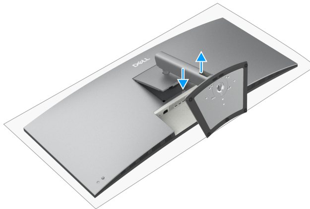
Figure 52. Removing the monitor stand
