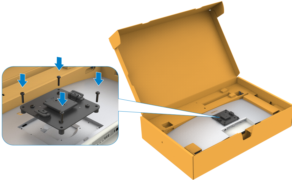
Figure 23. Attach the mounting bracket
