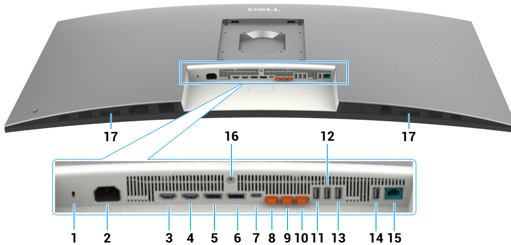
Figure 4. Bottom view
