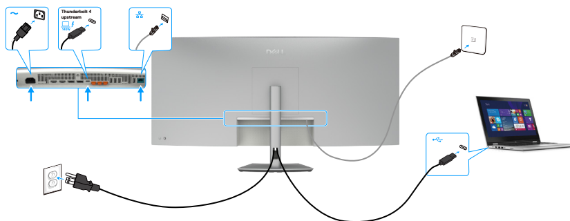
Figure 34. Network routing via Thunderbolt 4 upstream port
