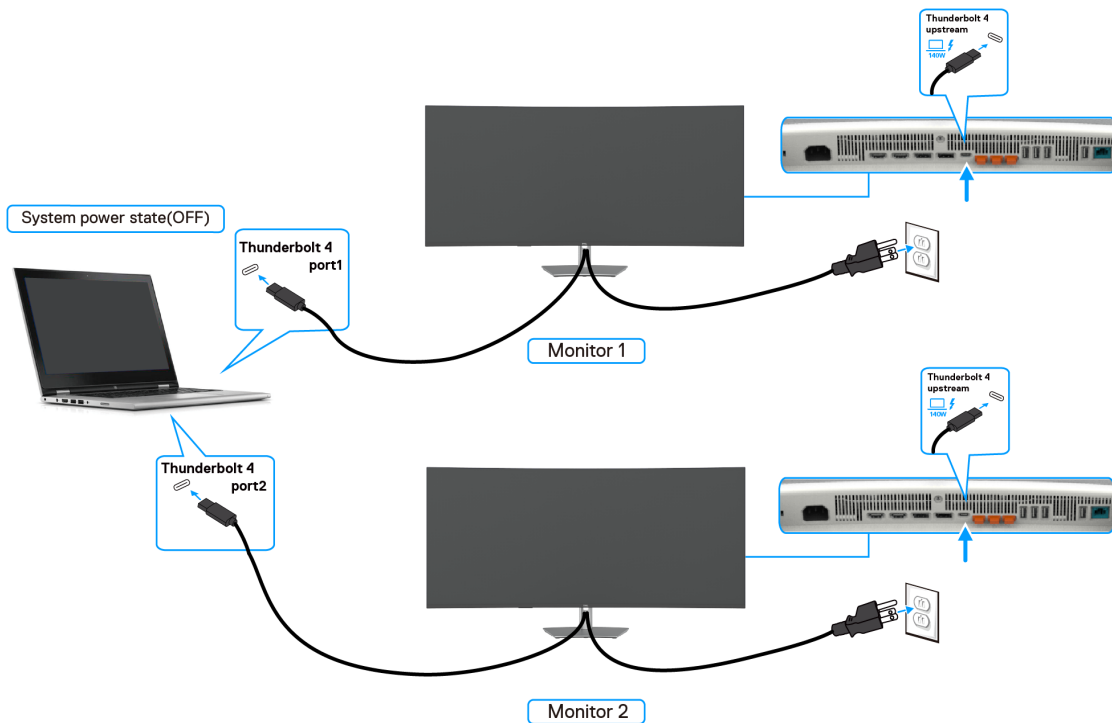
Figure 49. Two monitors and computer power state Off in DPBS mode
