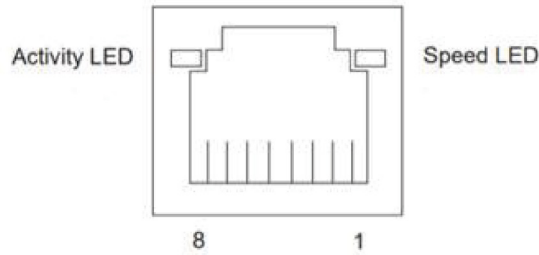
Figure 10. RJ45 Port (Connector Side)
