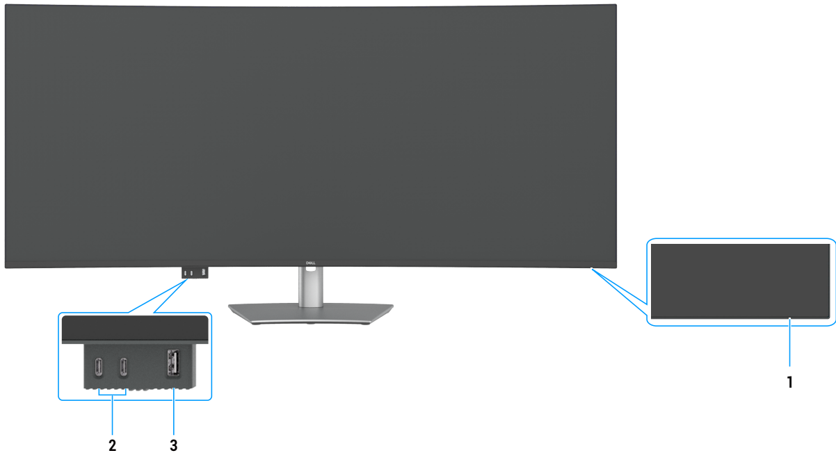
Figure 1. Front view
