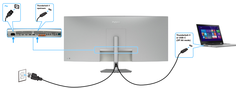
Figure 30. Connecting the Thunderbolt 4 cable
