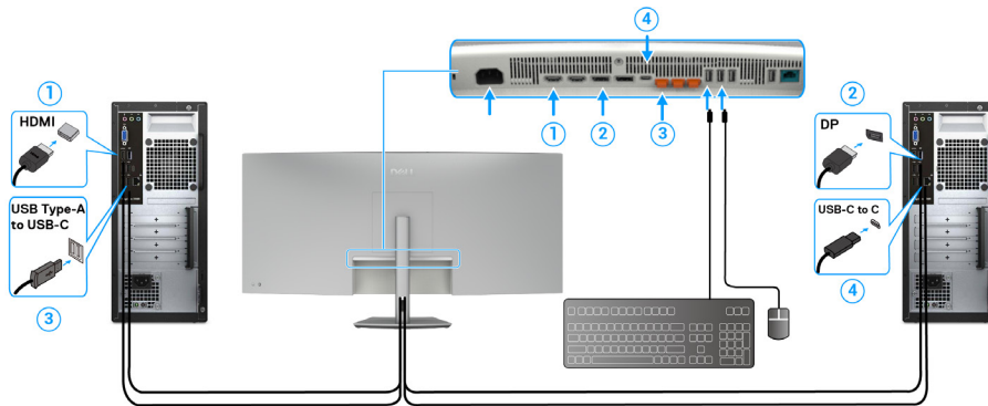
Figure 82. KVM 1 connecting
