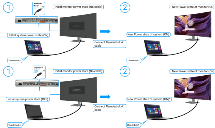
Figure 42. Dell Power Button Sync-Connect the Thunderbolt 4 cable
